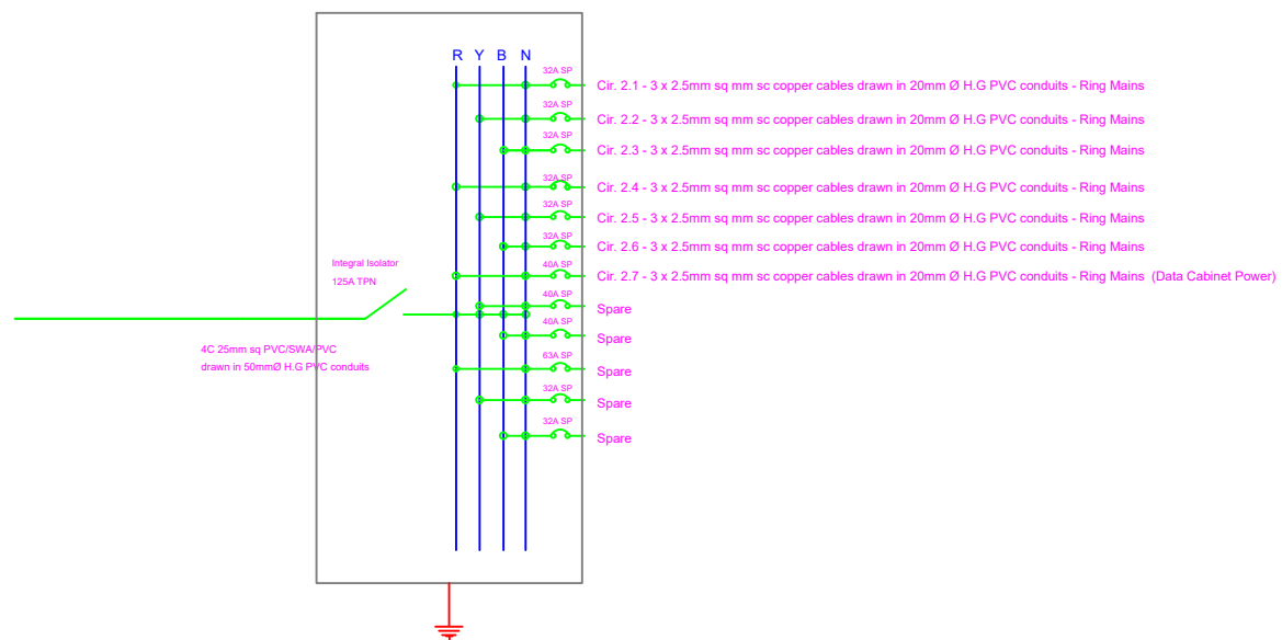
4 WAY DISTRIBUTION BOARD DB "2" AS SCHNEIDER FOR SURFACE MOUNTING
