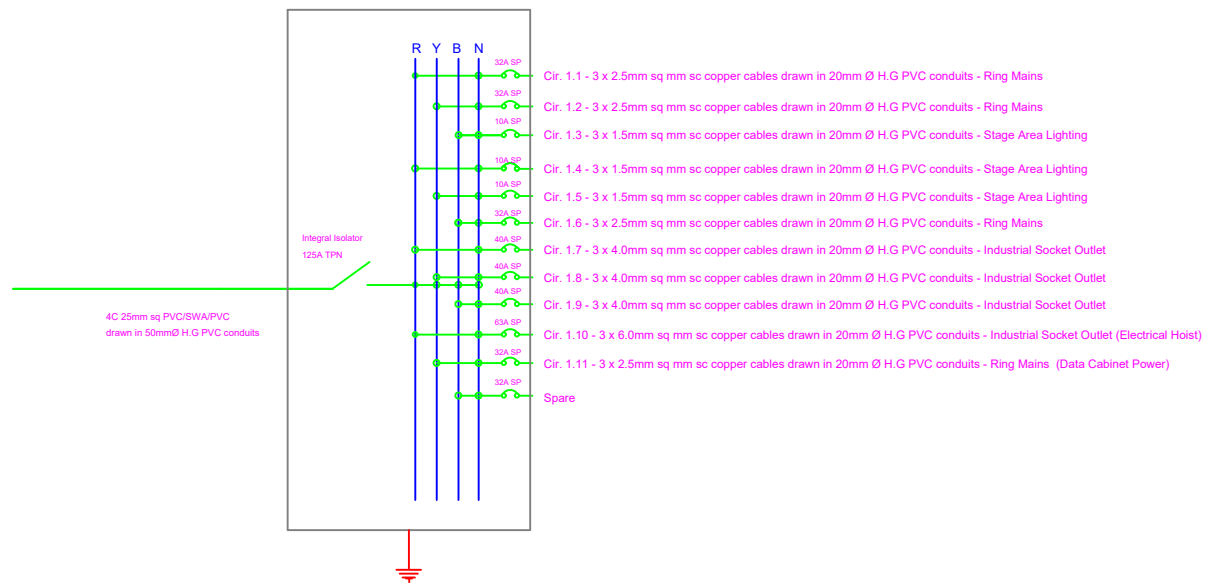
4 WAY DISTRIBUTION BOARD DB "1" AS SCHNEIDER FOR SURFACE MOUNTING
