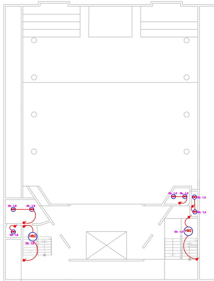
LIGHTING POINTS LAYOUT (LEVEL II)
