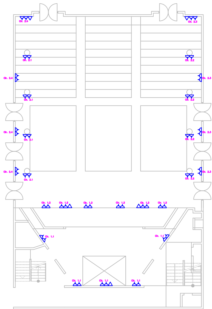
POWER POINTS LAYOUT (LEVEL I)
